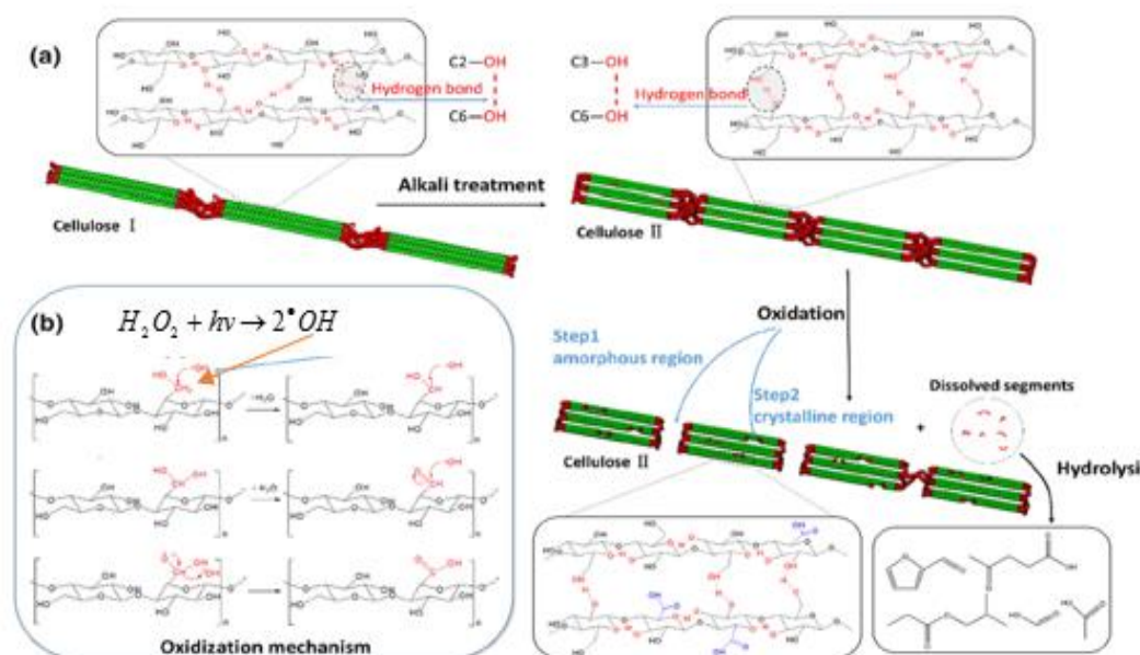
Fig. 4. Structure alteration of (a) cellulose, and (b) the oxidation mechanism
