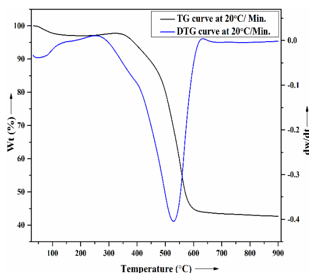
Fig. 1. TG-DTG plot of the coal sample at heating rate 20 °C/min
