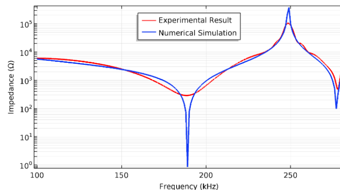
Fig. 8. Comparison between the experimental and the numerical simulation results of impedance-frequency curve for the piezoceramic elements
