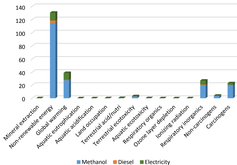
Fig 11. The results of applying the weighting coefficients of the IMPACT 2002+ method
