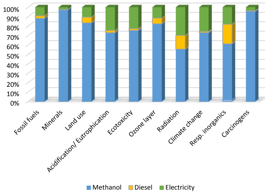
Fig .1. The results of applying the characteristic coefficients of the Eco-indicator 99 method
