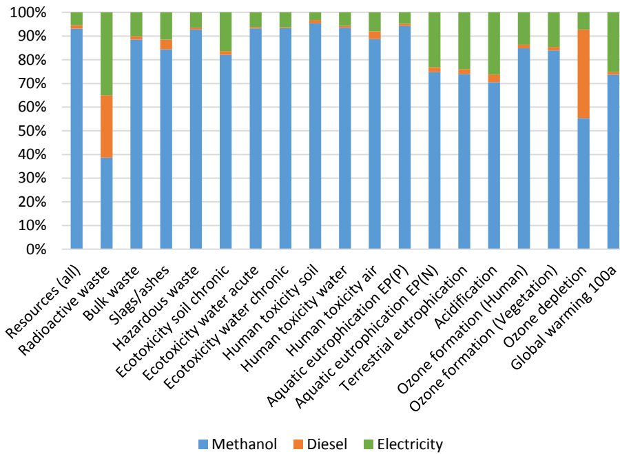
Fig.5. The results of applying the characteristic coefficients of the EDIP 2003 method.
