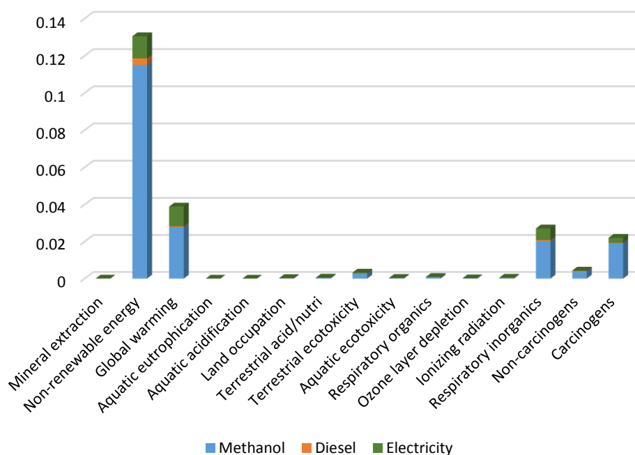
Fig.10. The results of applying the normalization coefficients of the IMPACT 2002+ method.
