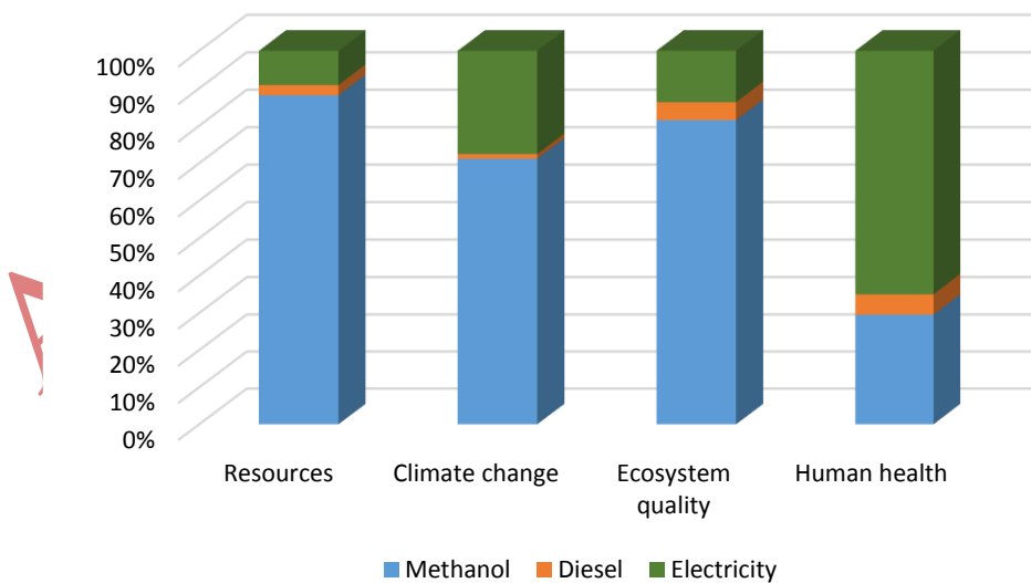
Fig.9. The results of applying the IMPACT 2002+ method
