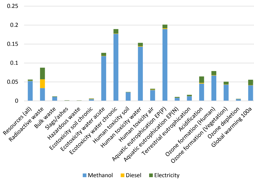
Fig.6. The results of applying the normalization coefficients of the EDIP 2003 method.
